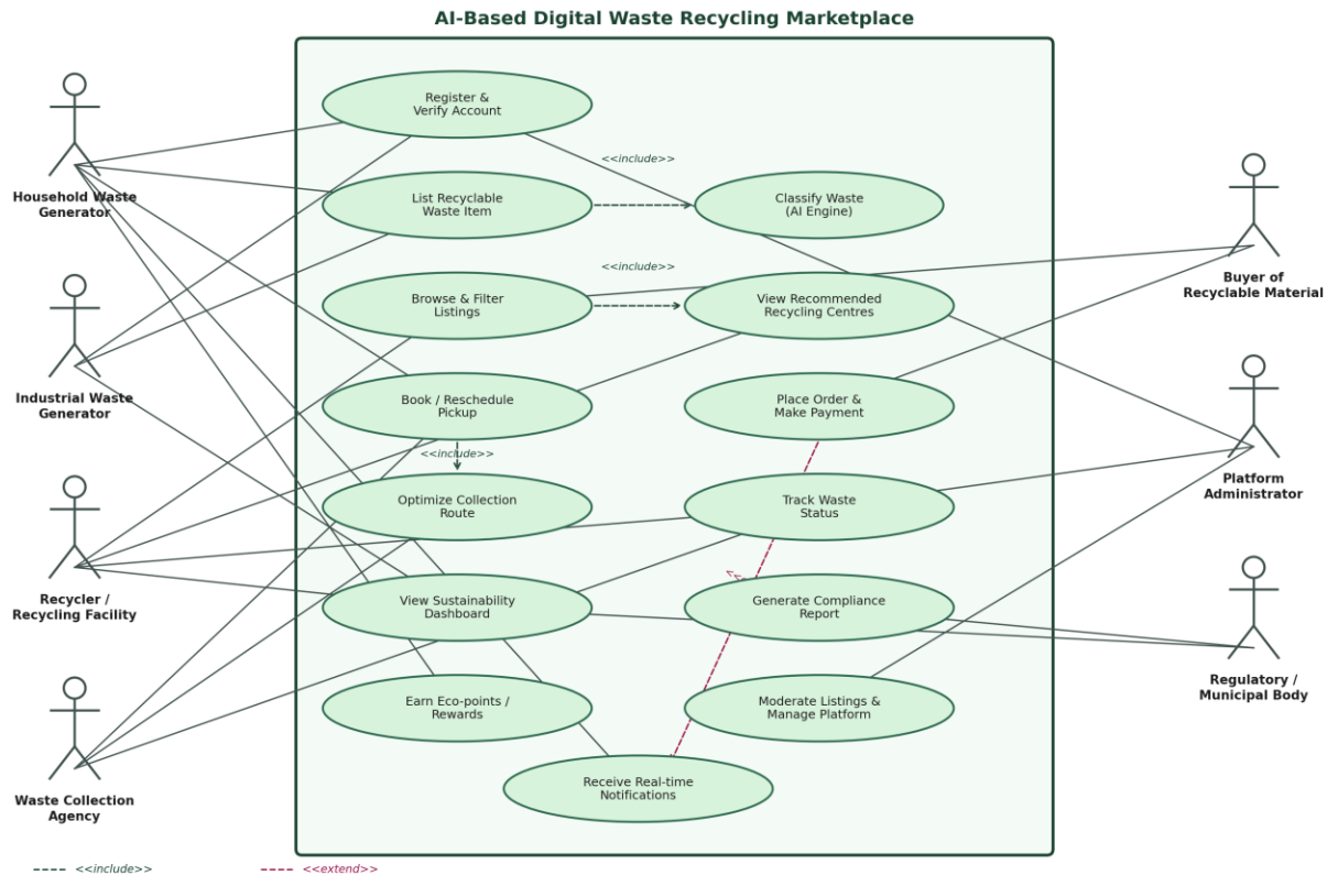
Figure 6.1 — UML Use Case Diagram: AI-Based Digital Waste Recycling Marketplace
